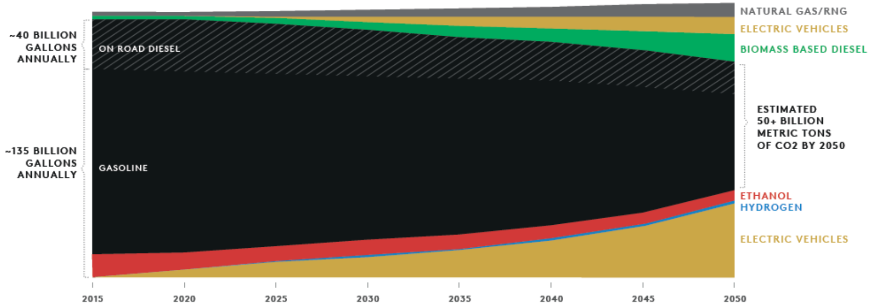
TRANSPORTATION TRANSITION IN QUADRILLION BTU 8,9,10,11
